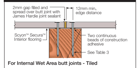
FIGURE 6 BUTT JOINING OPTIONS
